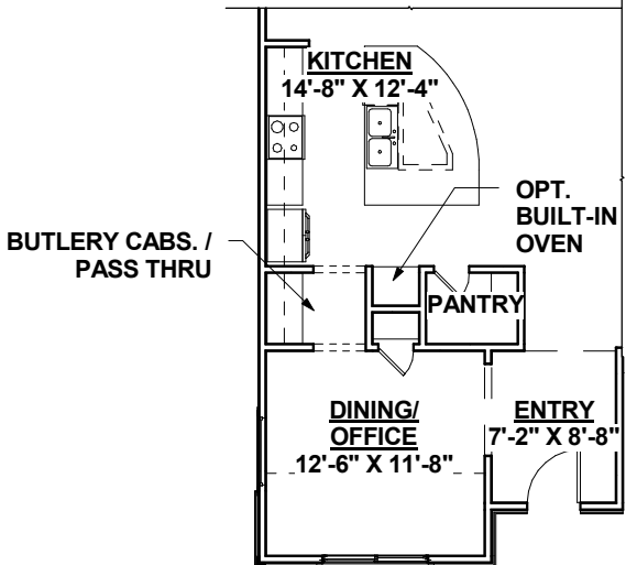
OPT. DINING KITCHEN LAYOUT - PASS THRU
