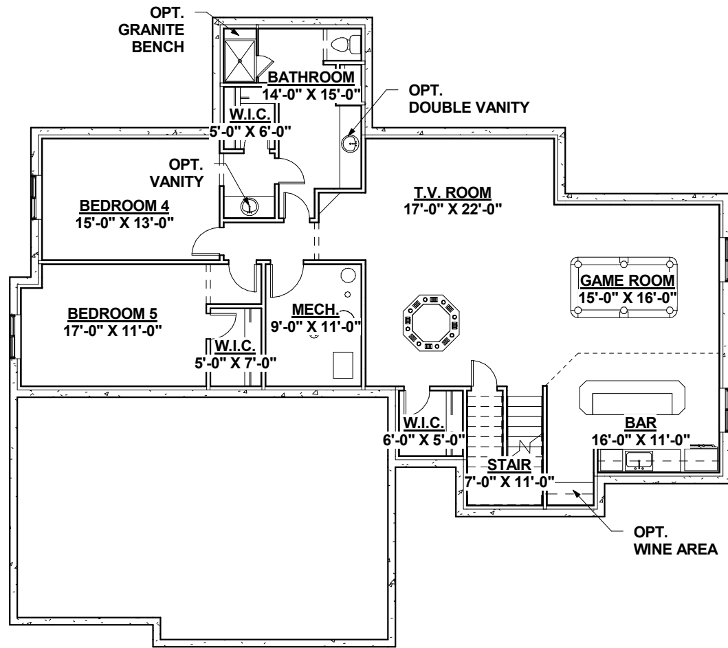
OPT. BASEMENT FINISH FLOOR PLAN
