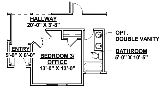
OPT. OFFICE LAYOUT
