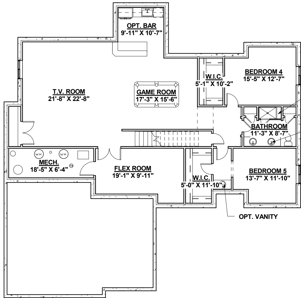
OPT. BASEMENT FINISH FLOOR PLAN
