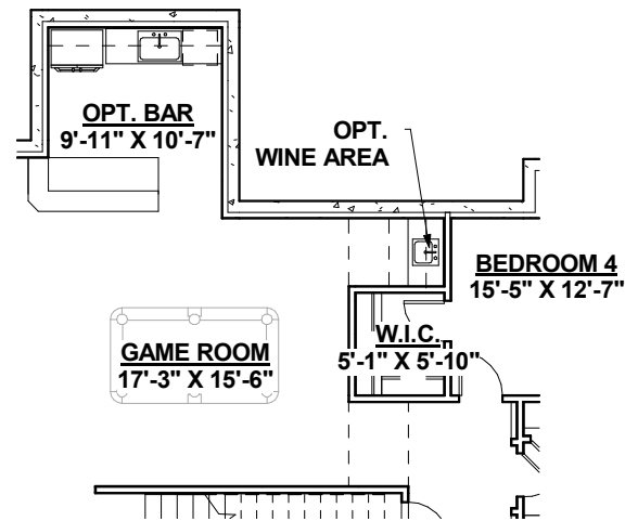
OPT. BASEMENT FINISH FLOOR PLAN - WINE AREA
