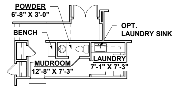
OPT. MUDROOM/ LAUNDRY LAYOUT
