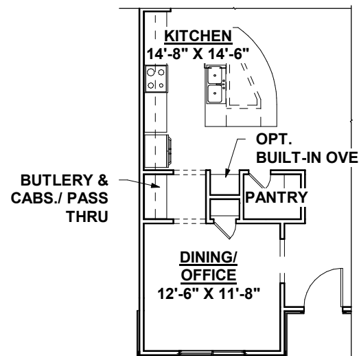
OPT. KITCHEN/ DINING LAYOUT 1
