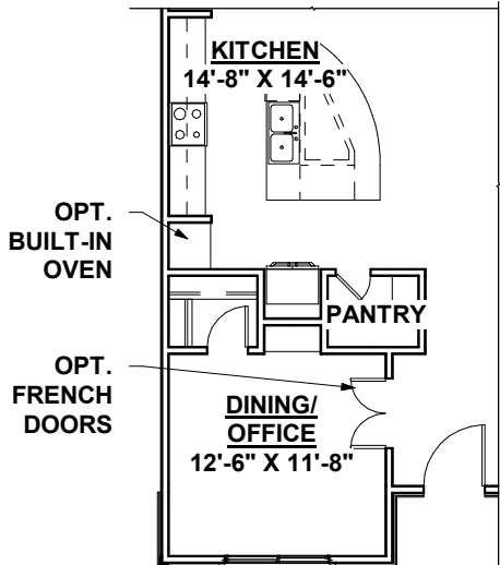
OPT. KITCHEN/ DINING LAYOUT 2
