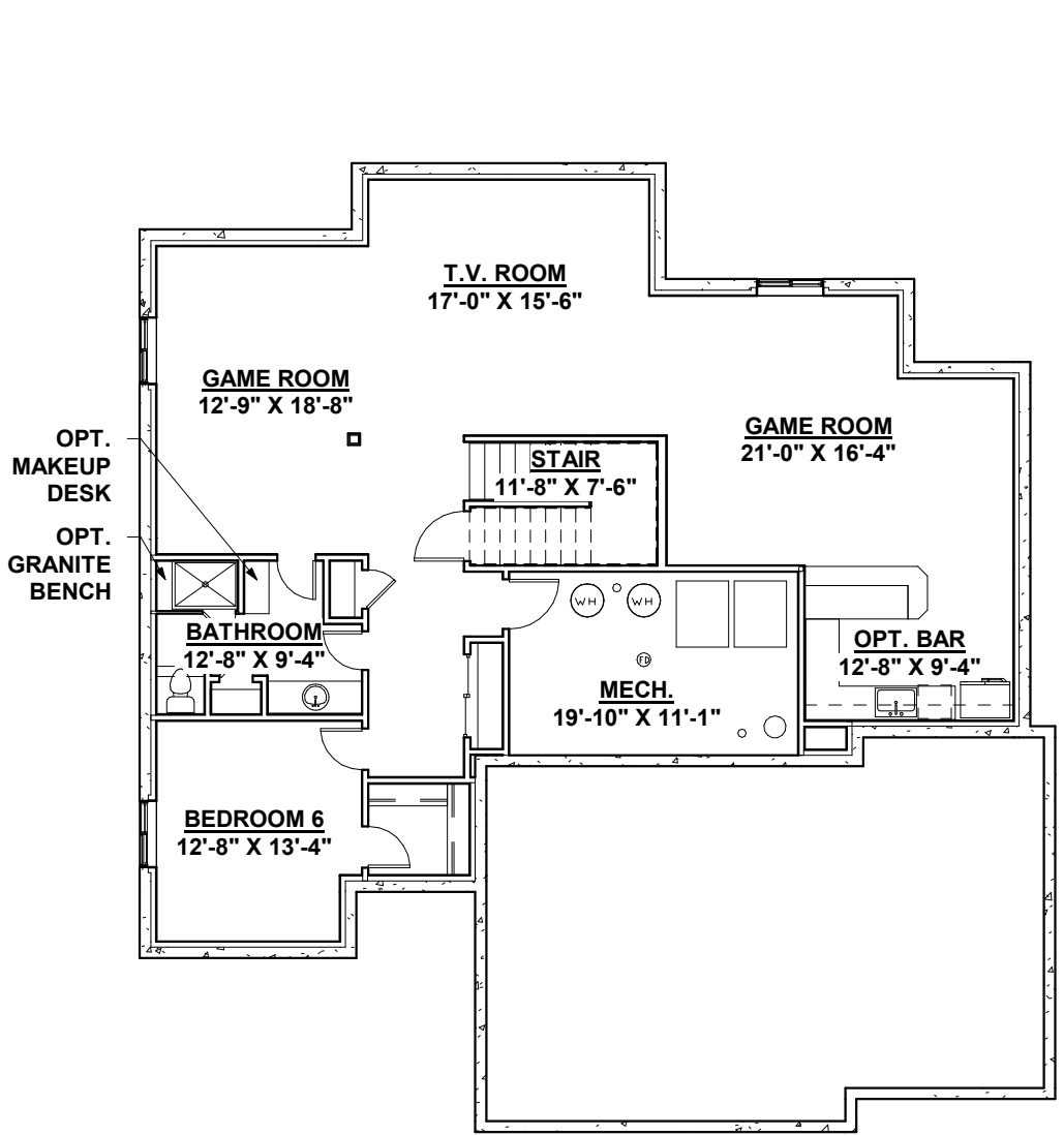
OPT. BASEMENT FINISH FLOOR PLAN
