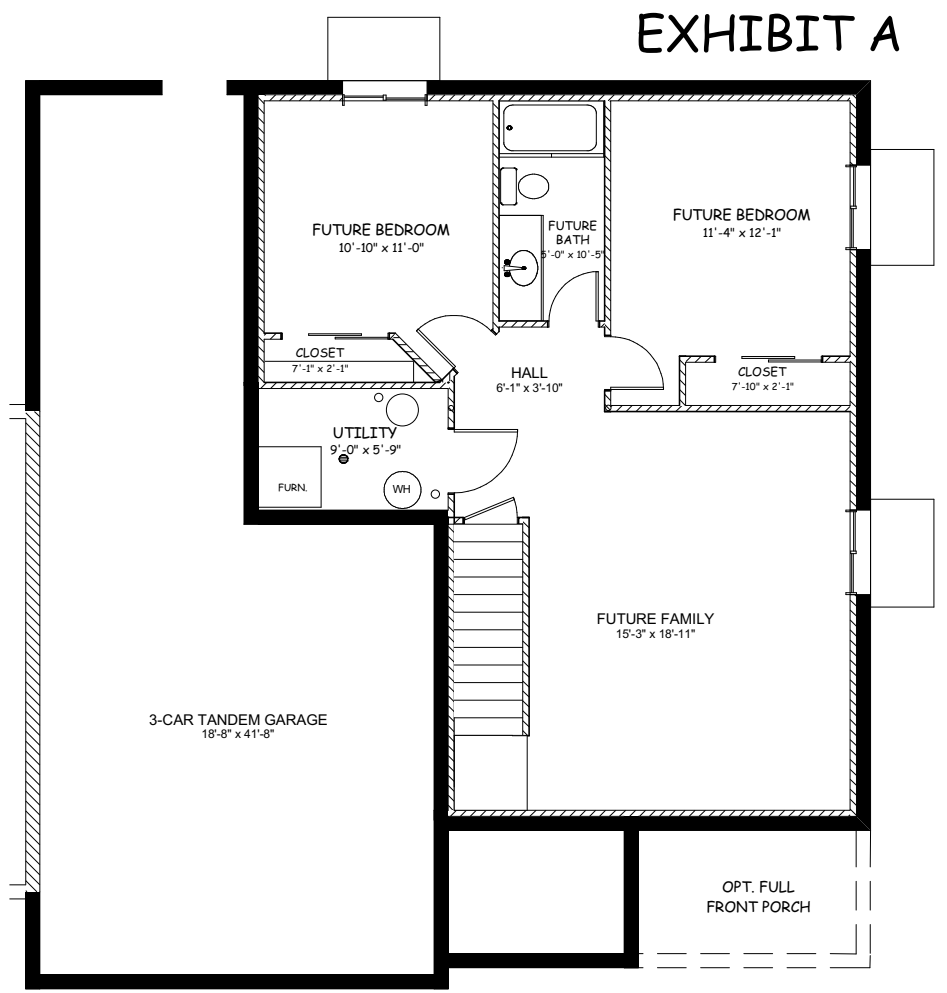
OPTIONAL BASEMENT FINISH
