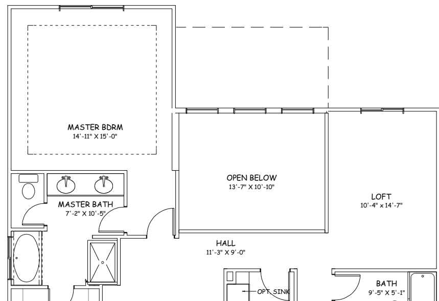
OPT. LOFT FLOOR PLAN
