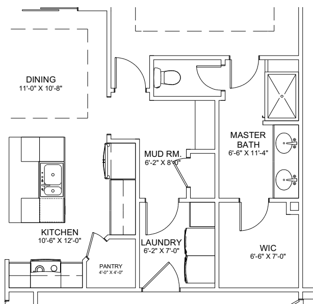
MASTER BATH/MUD ROOM OPTIONAL FLOOR PLAN 2
