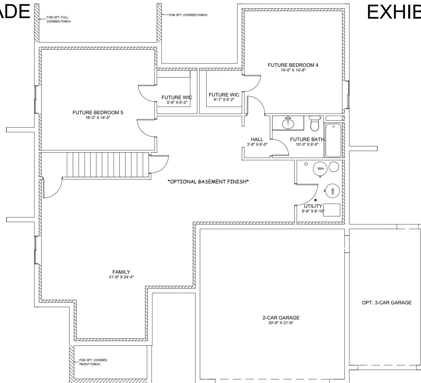
OPTIONAL BASEMENT FINISH PLAN
