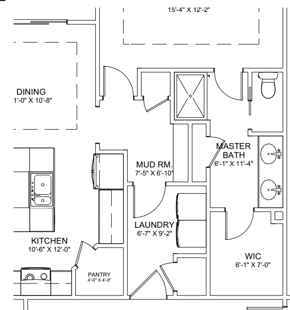
MASTER BATH/MUD ROOM OPTIONAL FLOOR PLAN 4
