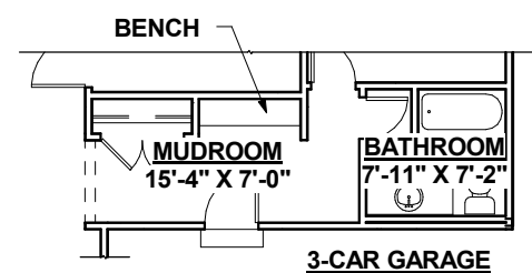
MUDROOM LAYOUT
