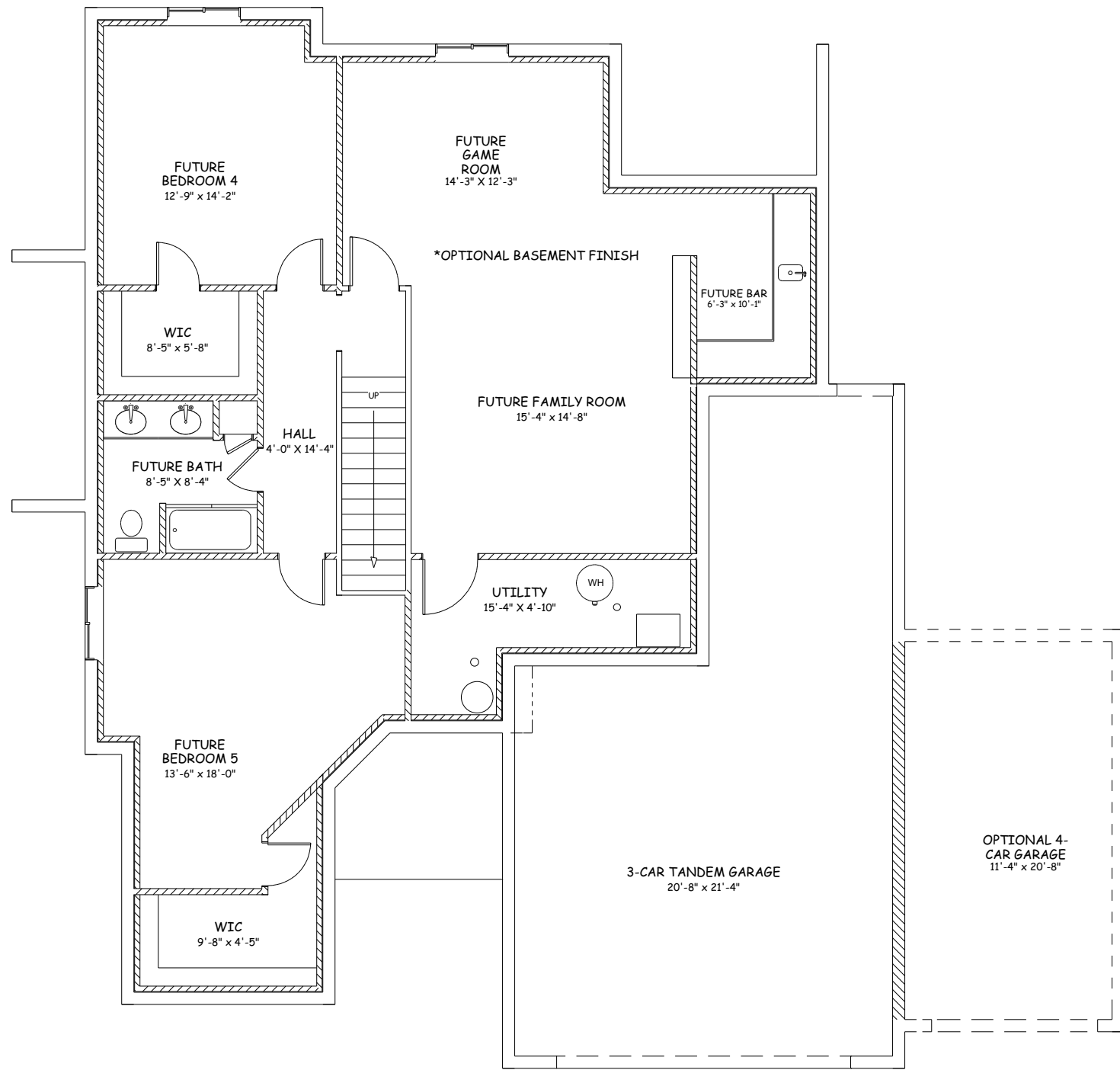
BASEMENT PLAN
