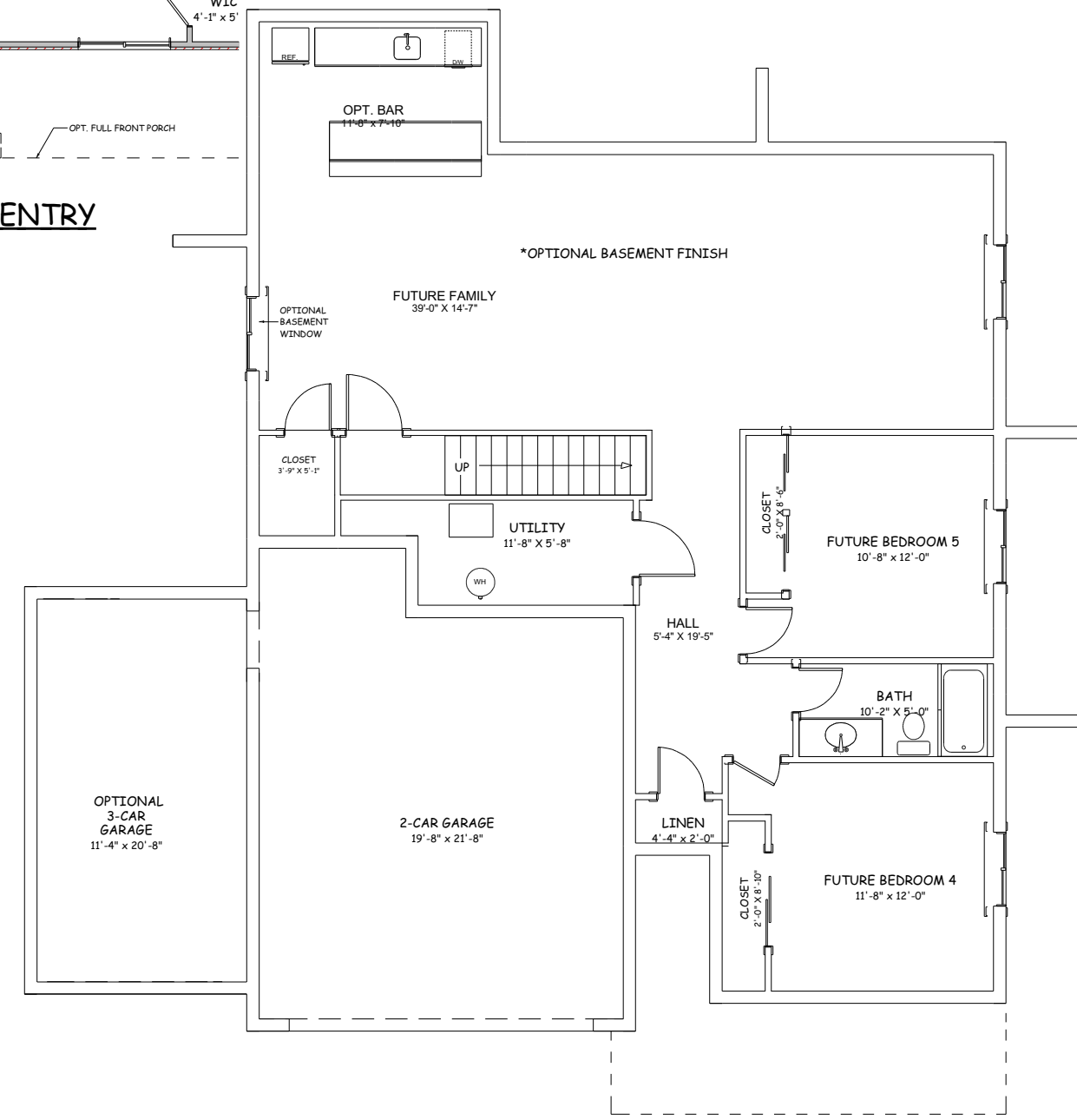
FOUNDATION PLAN
