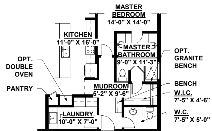
OPT. MUDROOM/ KITCHEN/ MASTER SUITE LAYOUT
