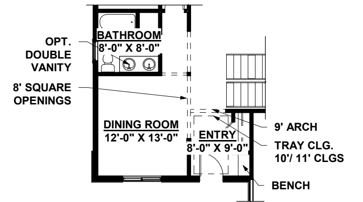
OPT. DINING ROOM LAYOUT
