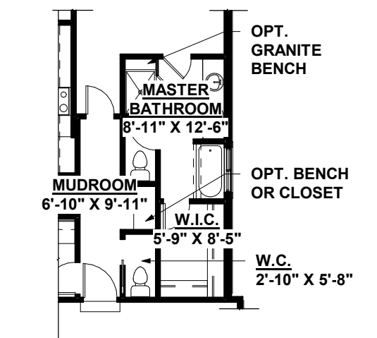
OPT. MUDROOM/ MASTER SUITE LAYOUT
