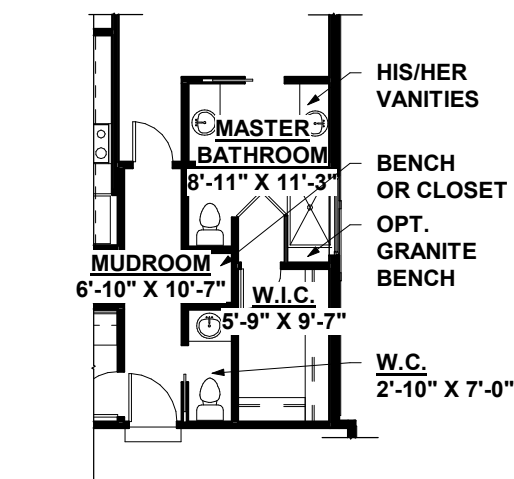
OPT. MUDROOM/ MASTER SUITE LAYOUT
