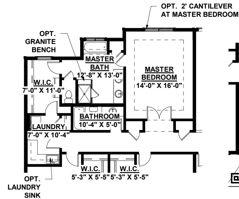
OPT. MASTER BEDROOM/ BATH/CLOSET/LAUNDRY AREAS
