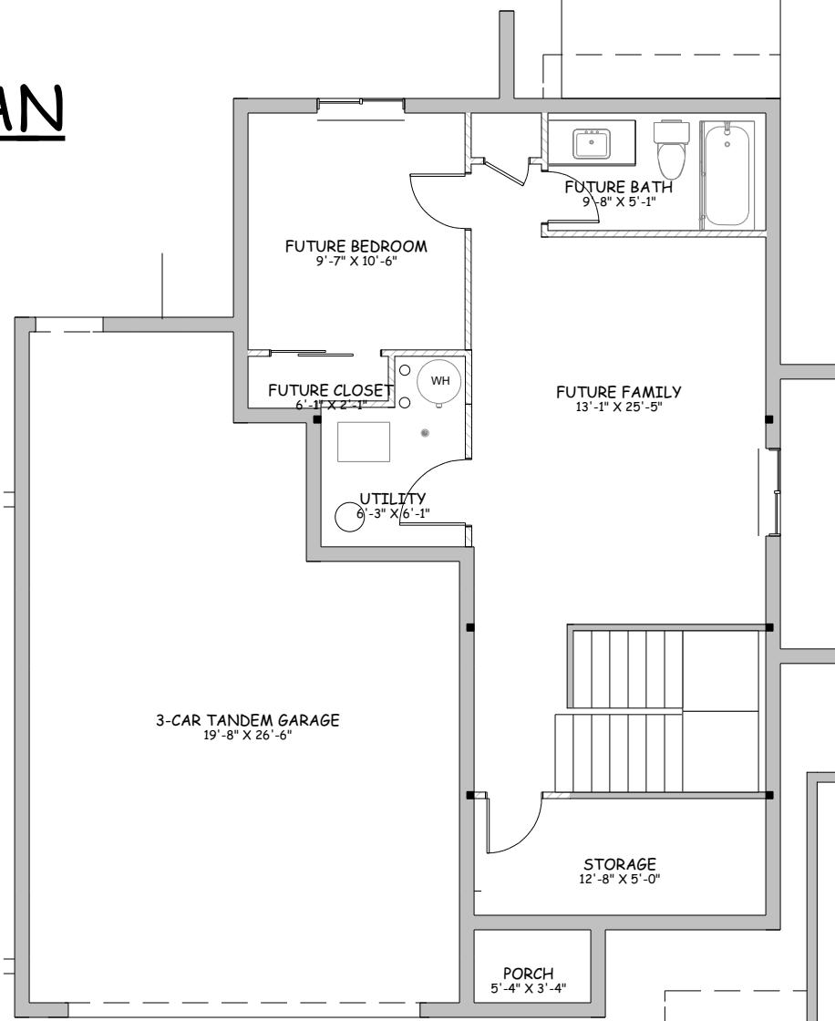
BASEMENT PLAN
