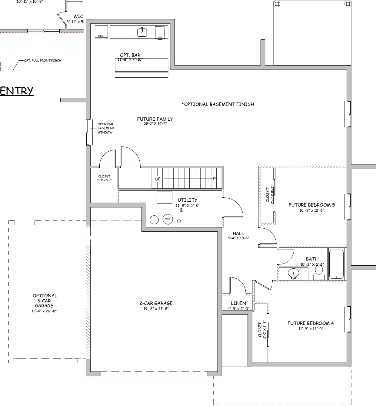
FOUNDATION PLAN
