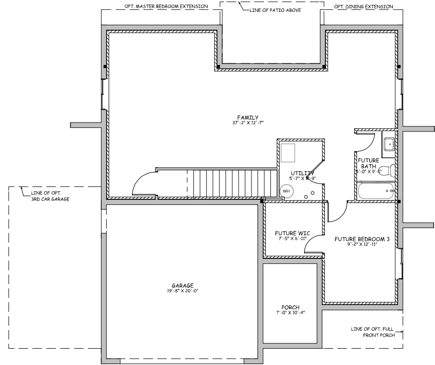
BASEMENT PLAN
