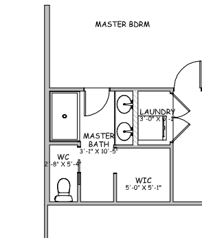
MASTER BATH OPTION 3
