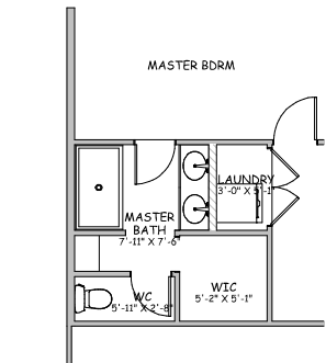
MASTER BATH OPTION 2
