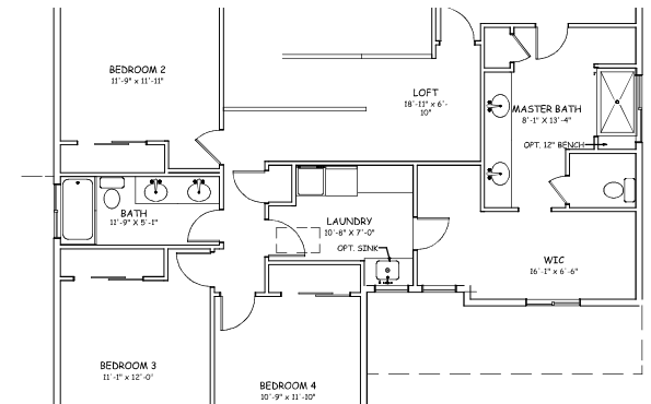
OPTIONAL LAUNDRY/MASTER BATH LAYOUT
