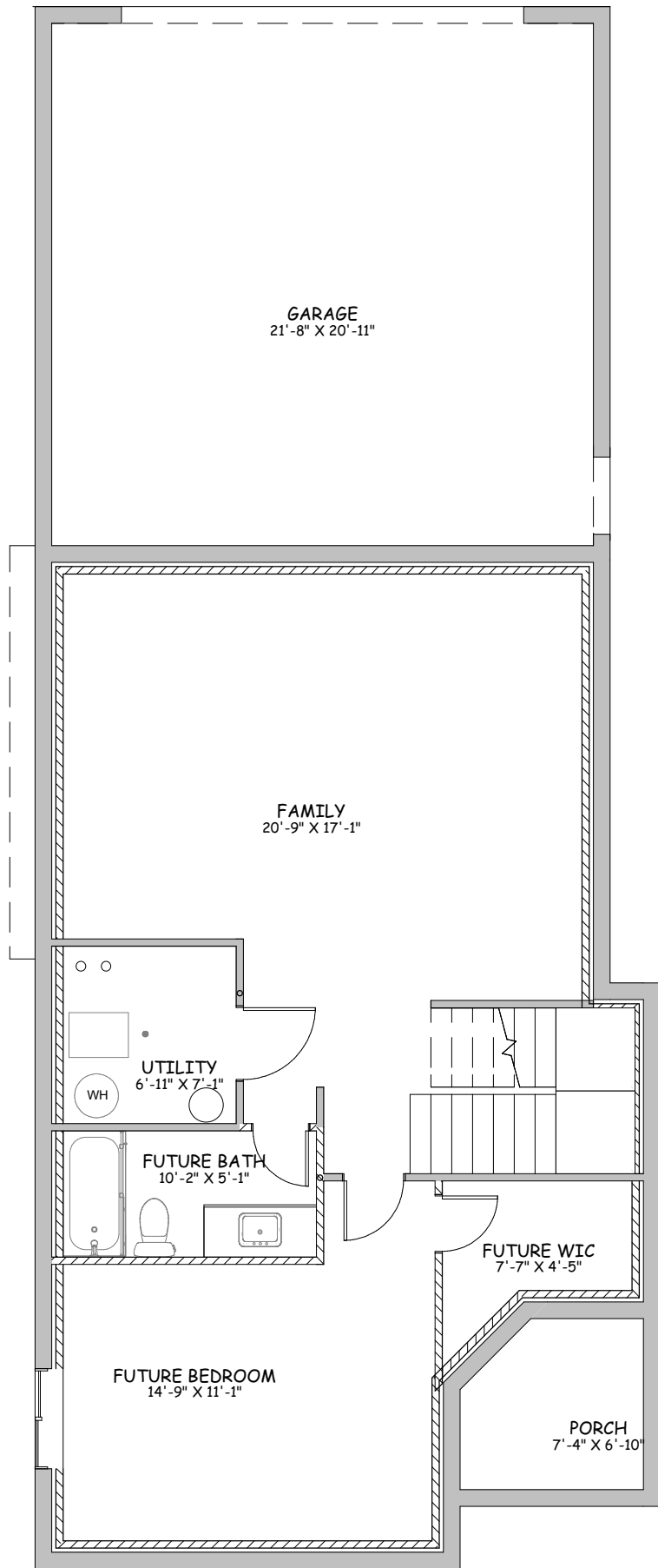
FUTURE BASEMENT PLAN
